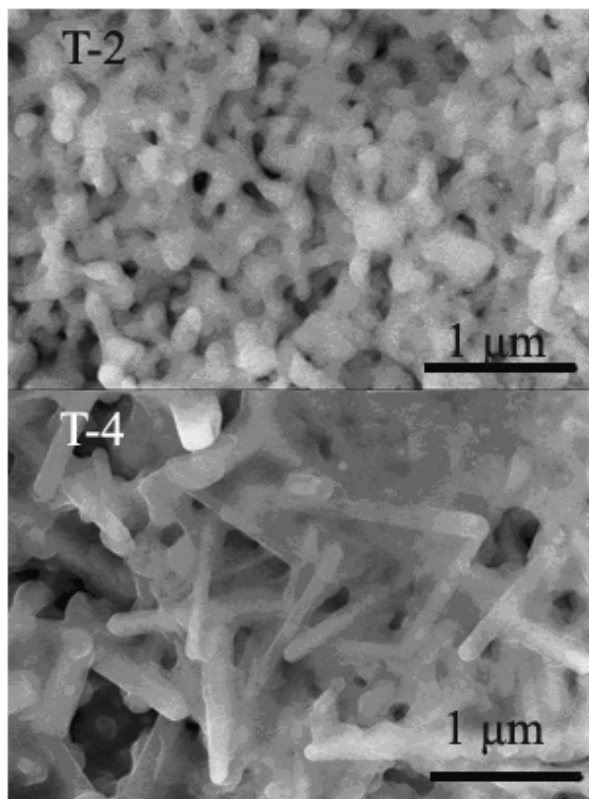
Fig. 1 SEM images of T-2/700 and T-4/700.
