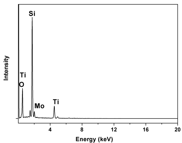
Fig. 2 The EDX spectrum of T-2.
