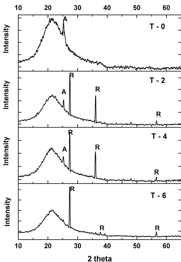
Fig. 3 XRD patterns of TiO 2 films undoped and doped with different amounts of Mo by thermal treatment at 500 °C. A: anatase, R: rutile.
