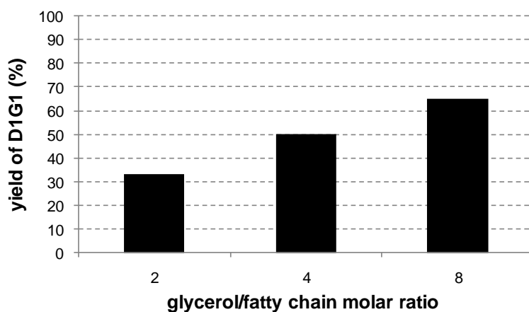
Figure S1: influence of the glycerol/fatty chain (1-dodecanol + 1-bromododecane) molar ratio on the D1G1 yield. Results were collected after 24h of reaction at 130°C
