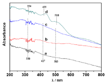
Fig. S3 UV-vis spectra of (a) 3a; (b) 3b; (c) 3c; (d) the neat chiral salen Mn(III) complex 2
