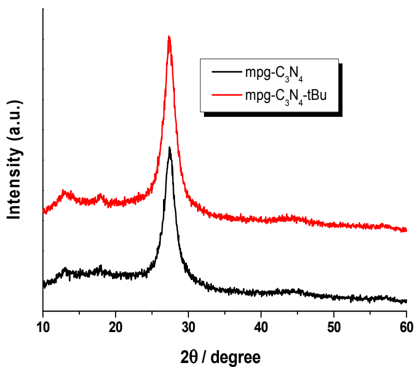
Figure S1: XRD patterns of mpg-C 3 N 4 and mpg-C 3 N 4 -tBu
