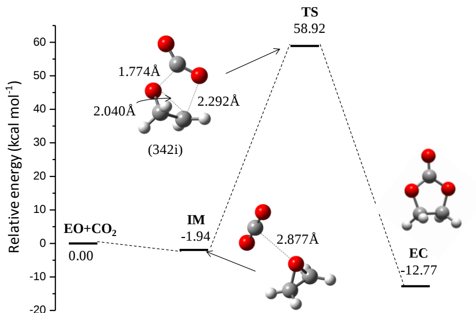
Fig. S1 Potential energy surface profiles for the cycloaddition reaction without catalyst.
