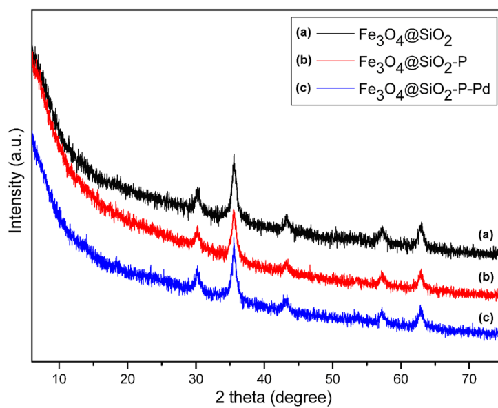
Figure S2. XRD of the supported Pd catalyst
