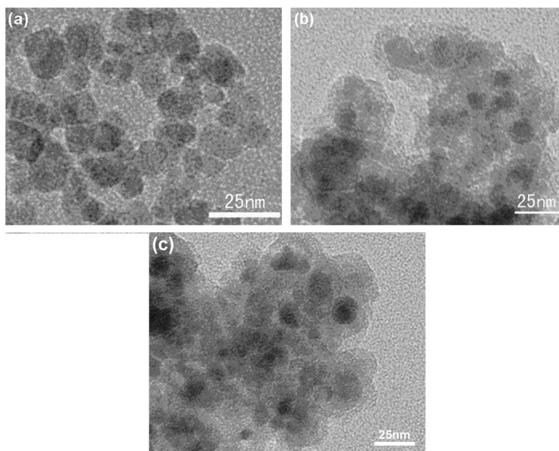
Figure S1. TEM images: (a) Fe 3 O 4 nanoparticles; (b) SiO 2 @Fe 3 O 4 ; (c) SiO 2 @Fe 3 O 4 -Pd catalyst
