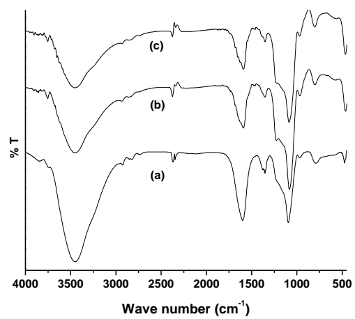
Fig. F FT-IR spectra of (a) 1% V_{imp} SiMCM-48, (b) 3% V_{imp} SiMCM-48, (c) 5% V_{imp} SiMCM-48
