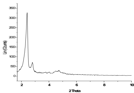
Fig. B XRD pattern of as synthesized CeMCM-48(Si/Ce 40)
