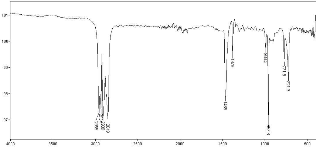
IR spectra of Xylyltrioxorhenium (solvent decane, decane subtracted).
