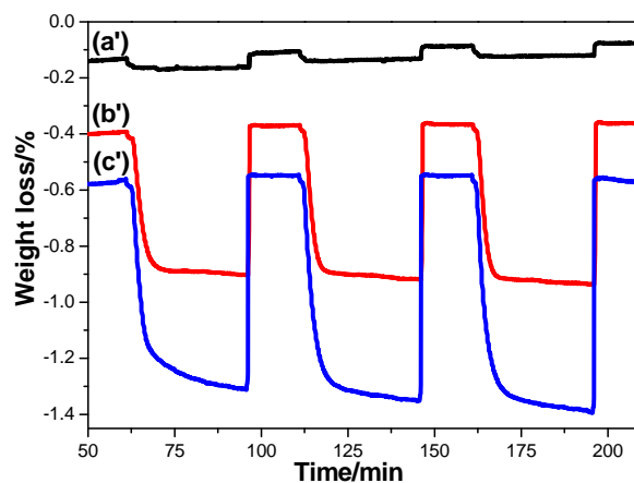
Figure S3. OSC of catalysts. (a') C, (b') CZ, (c') CZS
