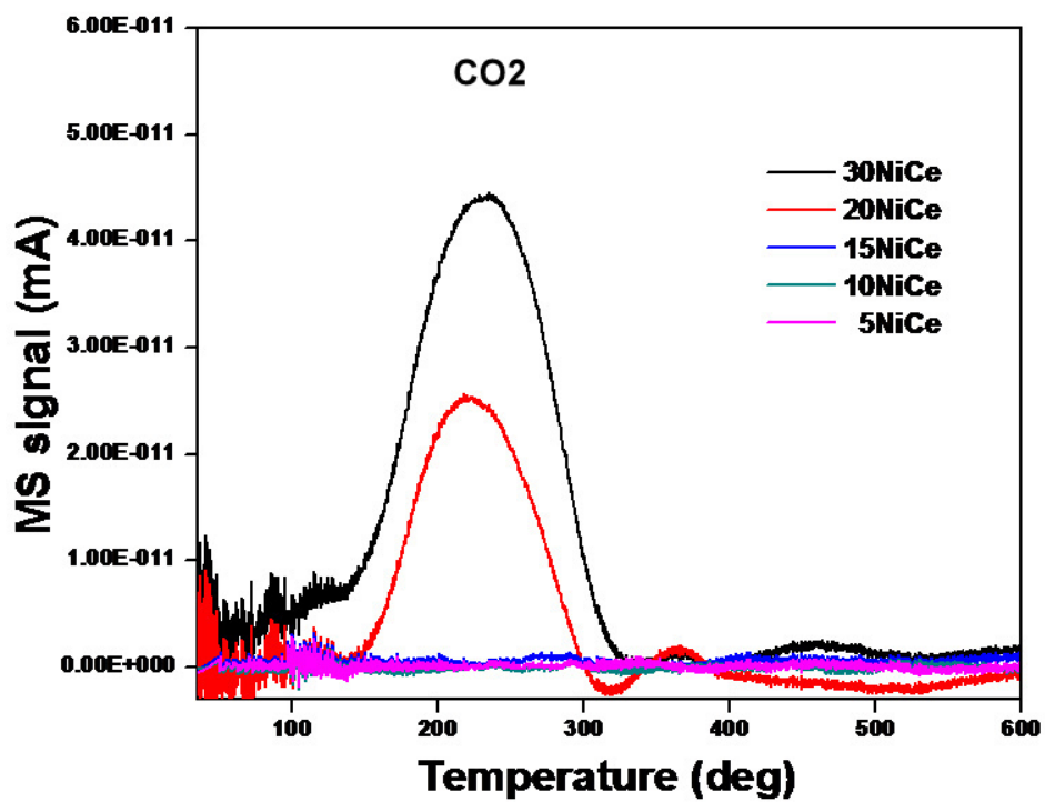
Fig S2: Temperature programmed decomposition of spent catalysts
