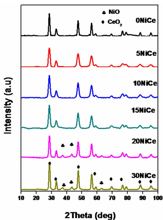
Fig S1. XRD patterns of the spent catalysts
