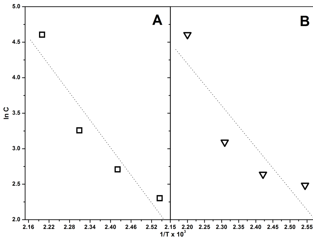
Figure S1. Arrhenius plots for the transesterification reactions on the catalysts (A) \text{ZnAl}_2\text{O}_4 and (B) \text{ZnFe}_2\text{O}_4 .
