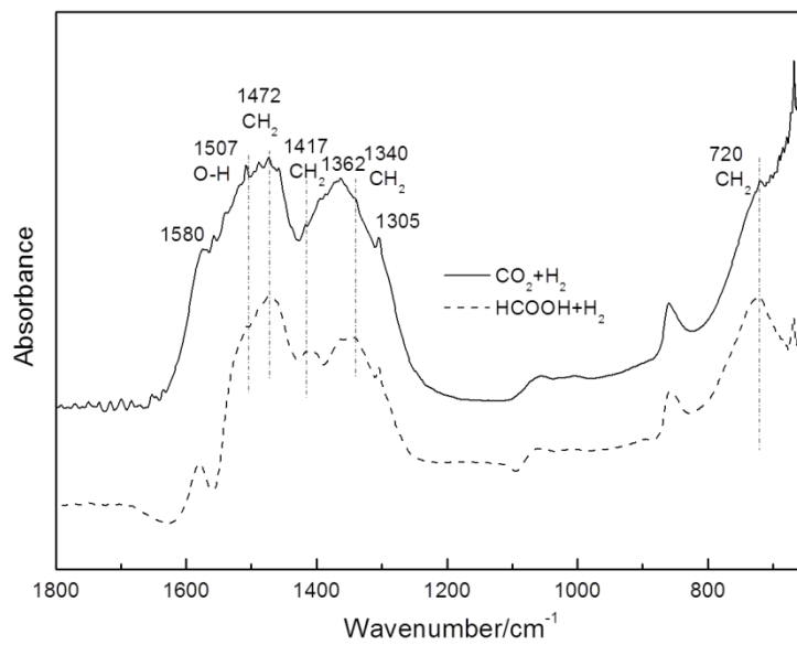
Figure s1. In-situ FTIR studies of \text{CO}_2 methanation and \text{HCOOH} hydrogenation on \text{Ni/Ce}_{0.5}\text{Zr}_{0.5}\text{O}_2 at 375^\circ\text{C} .
