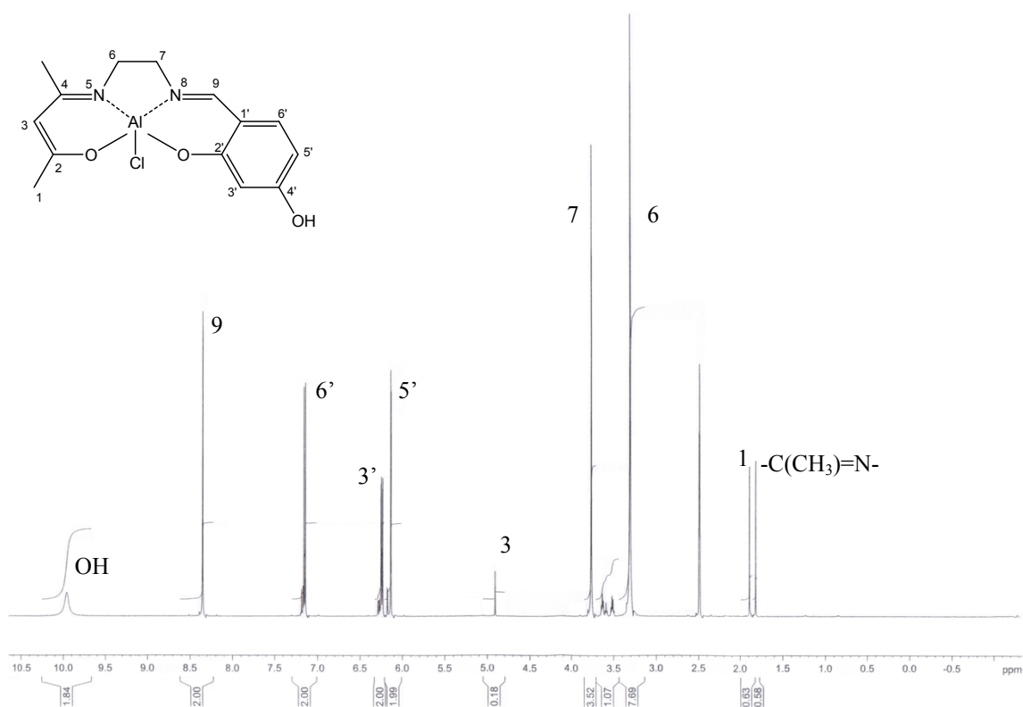
ESI Fig 1.2: 1 H NMR spectrum of Al1cat in DMSO
