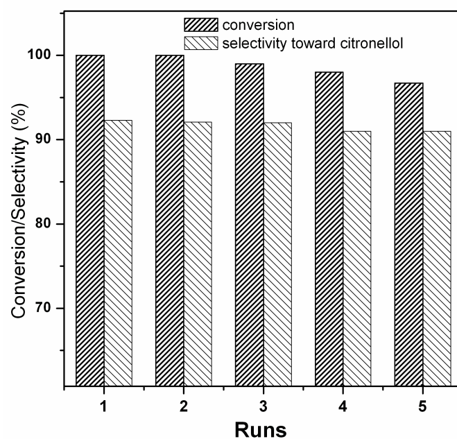
Fig. S1. The reusability of the Ni-ZnO(2)/C catalyst.
