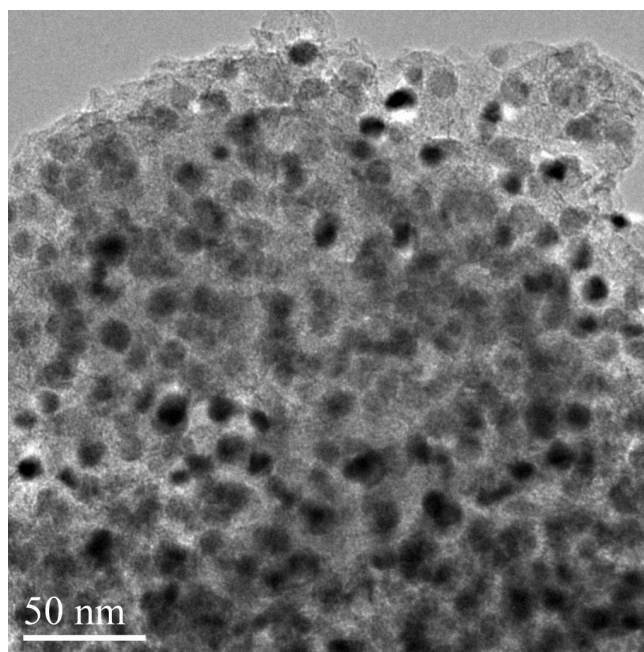
Fig. S2 TEM image of used Ni-ZnO(2)/C catalyst
