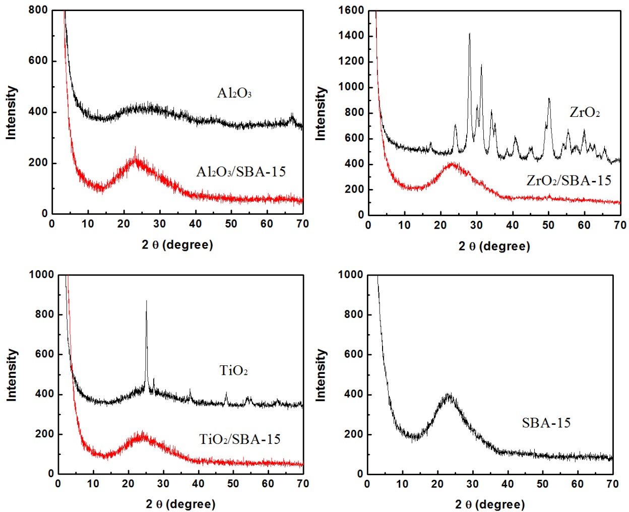
Figure S2. XRD spectra of metal oxide catalysts and SBA-15.
