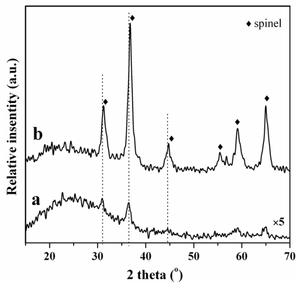
Fig.S1 XRD patterns of Im-MMO-0.5/A (a) and MMO-0.5 (b)
