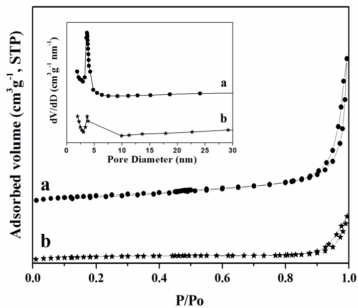
Fig.S2 Nitrogen adsorption–desorption isotherms of MMO-0.5 (a) and Im-MMO-0.5/A (b). Inset shows the pore size distributions.
