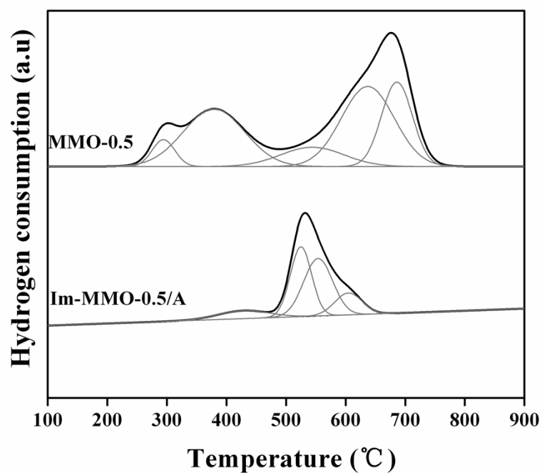
Fig.S3 H 2 -TPR profiles of comparison samples.
