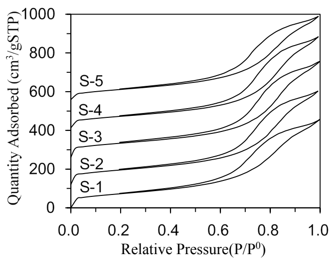
Figure S1. N 2 adsorption/desorption isotherms for different supports.
