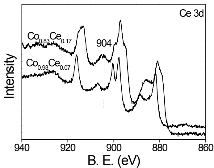
Fig. S1 XPS data for Ce 3d spectrum of \text{Co}_{0.93}\text{Ce}_{0.07} and \text{Co}_{0.83}\text{Ce}_{0.17} .
