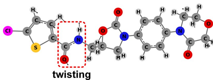
Fig. S1. Molecular motion of rivaroxaban, corresponding to the experimental THz peak at 2.17 THz
