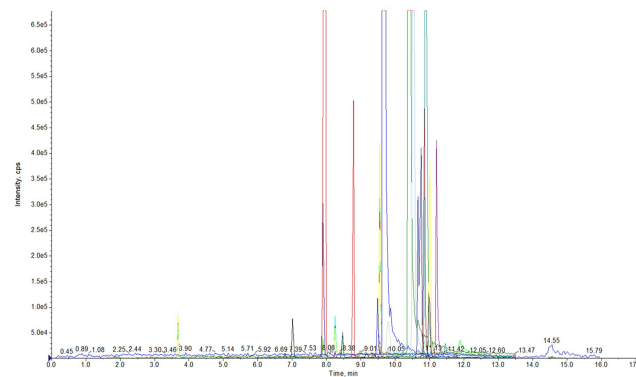
E 20 mM NH 4 COOH pH=6.36
