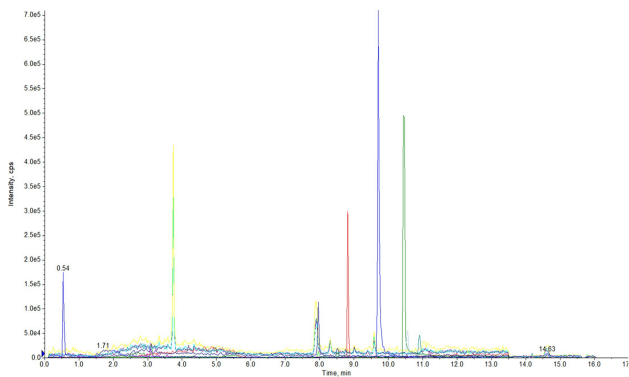
D 0.02% FA pH=3.75
