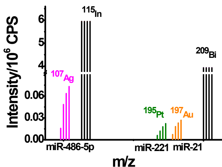
Figure S1. ICP-MS mass spectrogram of the multiplexed miRNAs in the serum with the concentrations of 0 pM (blank sample), 1 pM, 10 pM and 50 pM. (The internal standard concentration of ^{115}\text{In} and ^{209}\text{Bi} are 1.0 mg/L)
