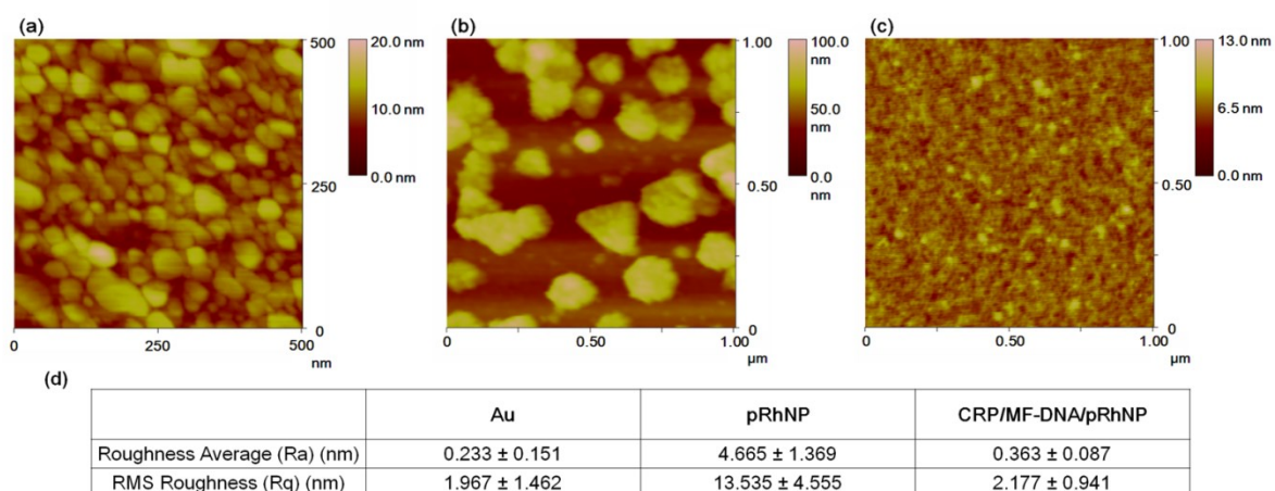
Fig. S1. Surface morphology of (a) bare Au substrate, (b) pRhNP and (c) CRP-immobilization on MF-DNA/pRhNP heteroalyer substrate, (d) Surface roughness analysis of each layer
