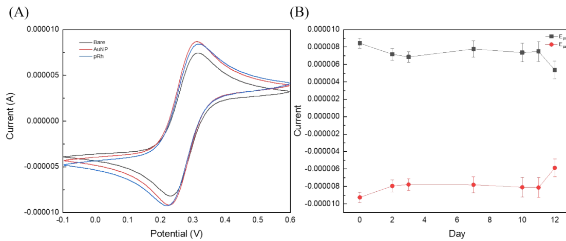
Fig. S2. (A) Comparison of electrical activity between commercially available gold nanoparticles and pRh. (B) Durability test of pRh.
