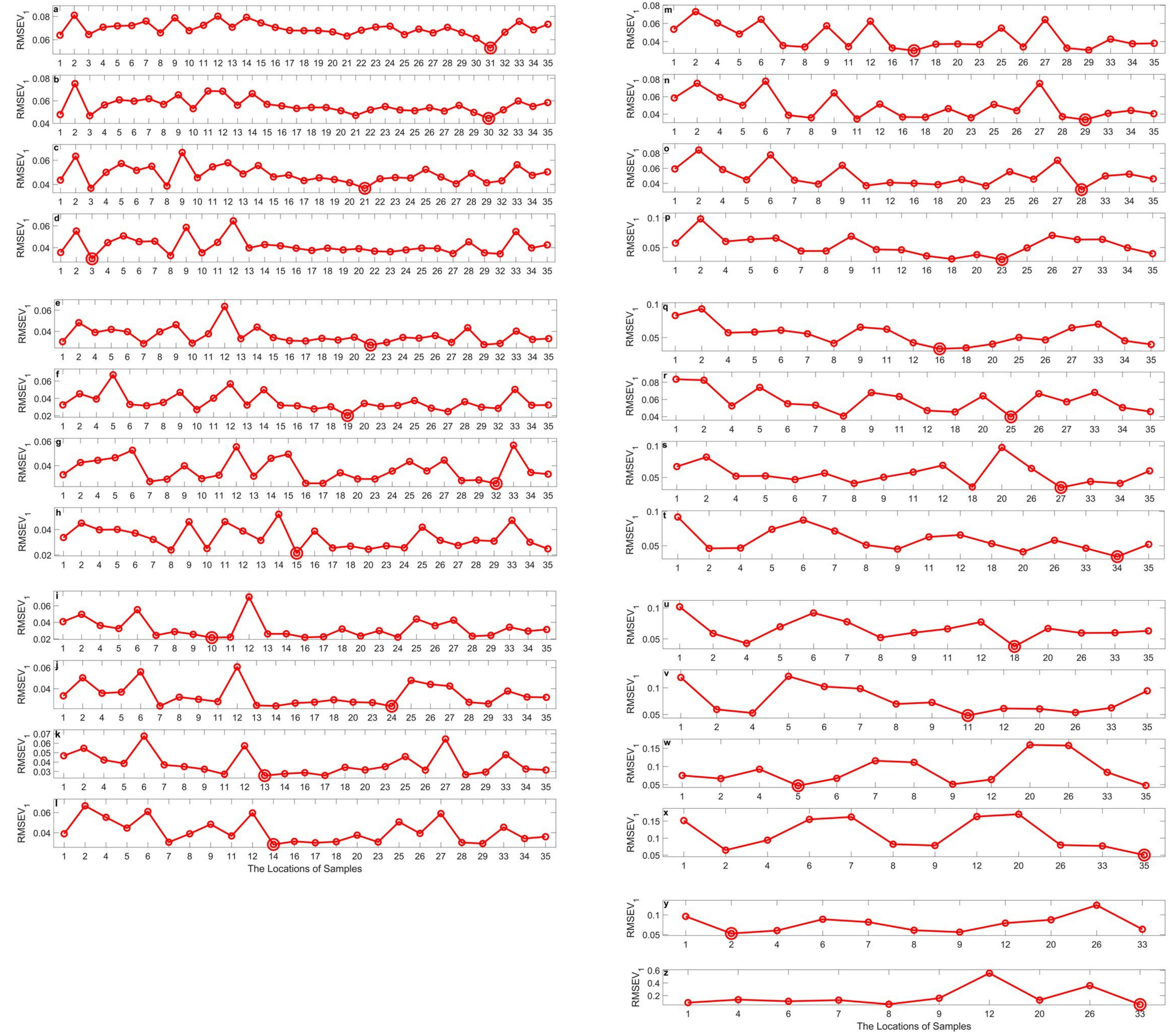
The RMSEV 1 values of CCA-ICE at omitting each sample at outer loops from m 2 =1 to 26 (from plots a to z) under m 1 =35
