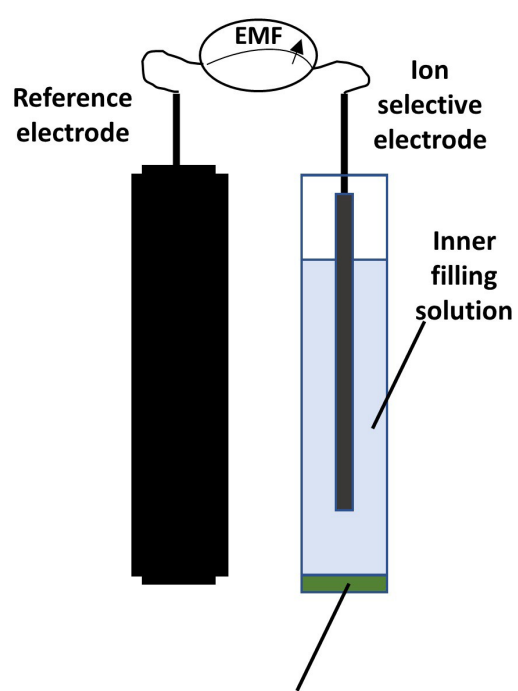
Sensor VII Conventional liquid contact ISE
