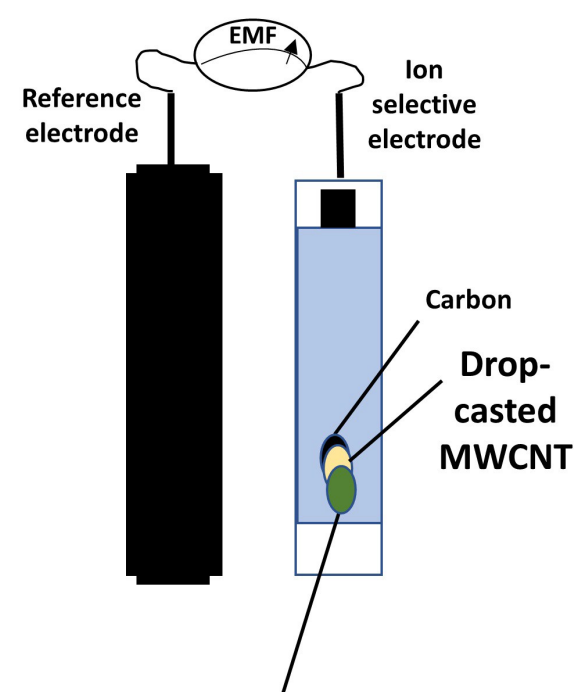
Sensor XIII Carbon Screen printed electrode + MWCNT + ISM
