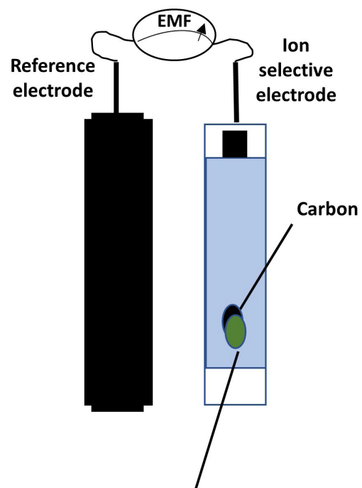
Sensor XII Carbon Screen printed electrode + ISM
