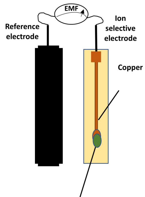
Sensor XI Cu-microfabricated electrode + ISM
