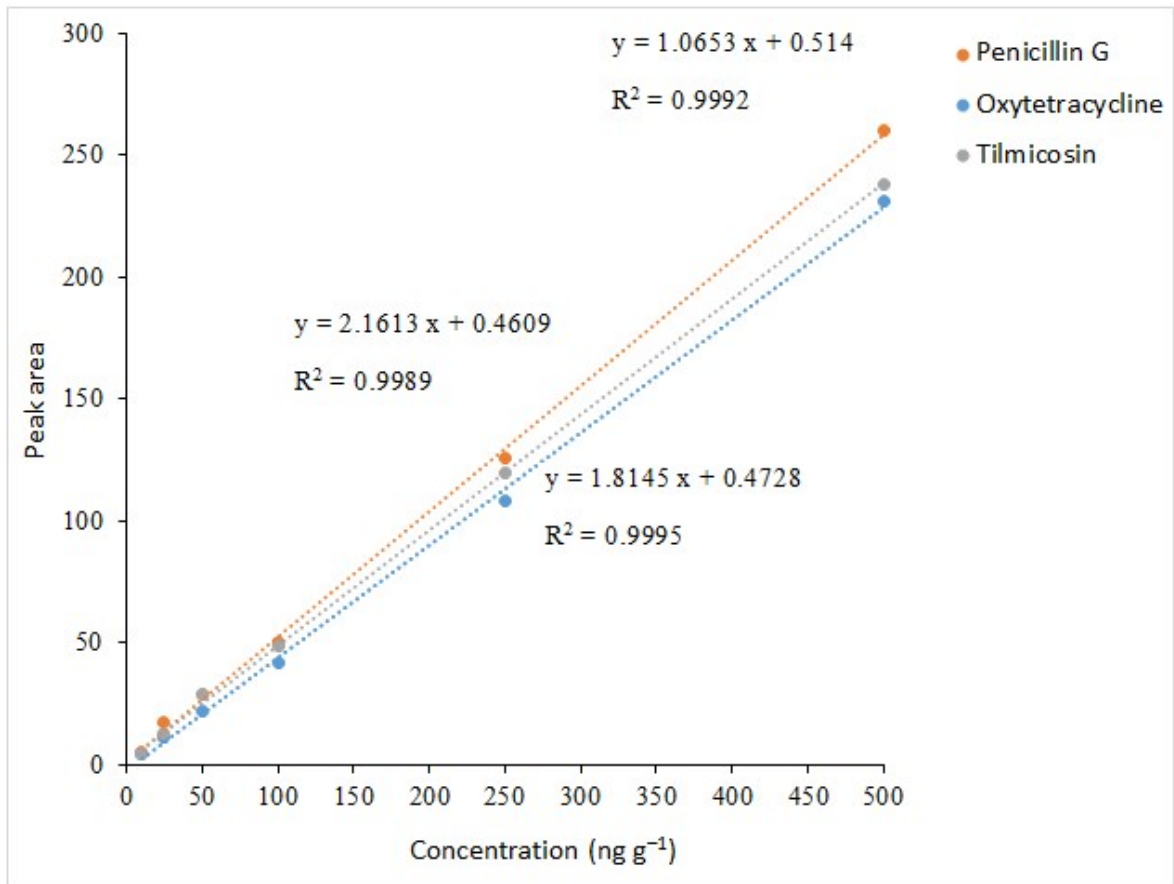
Fig. S2. Calibration curves for the studied analytes.
