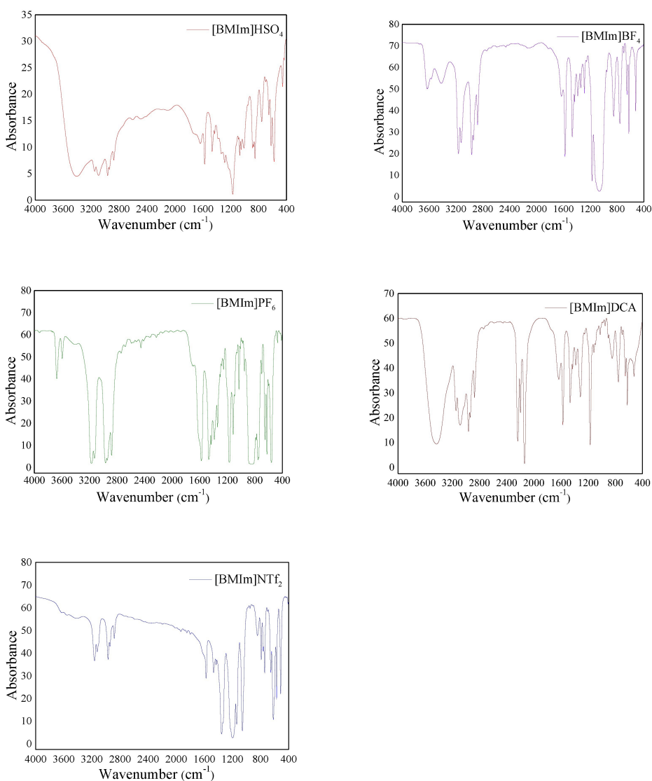
Fig. S1 FT-IR spectra of [BMIm]HSO 4 , [BMIm]DCA, [BMIm]PF 6 , [BMIm]BF 4 and [BMIm]NTf 2
