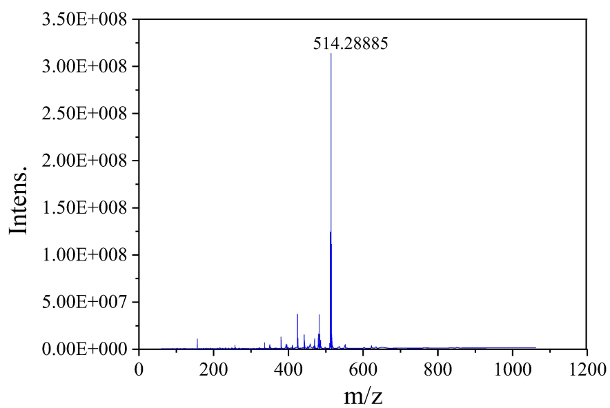
Fig. S10 ESI-MS spectrum of SRB-NB
