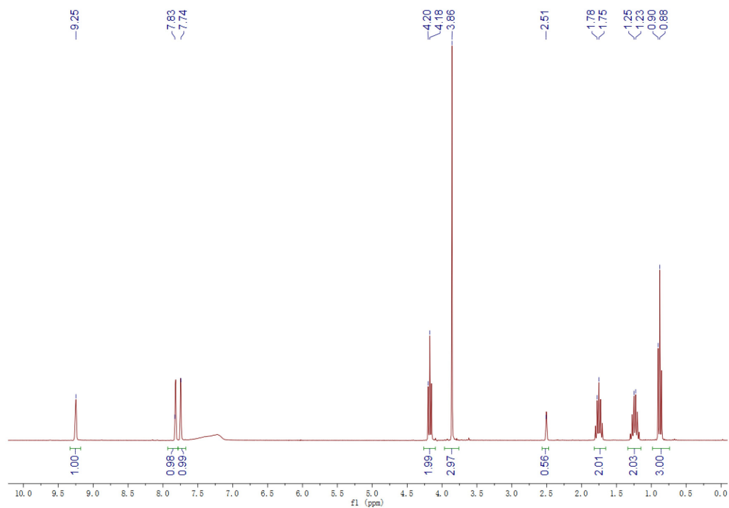
Fig. S2 ^1\text{H} NMR spectrum of [BMIm]HSO 4
