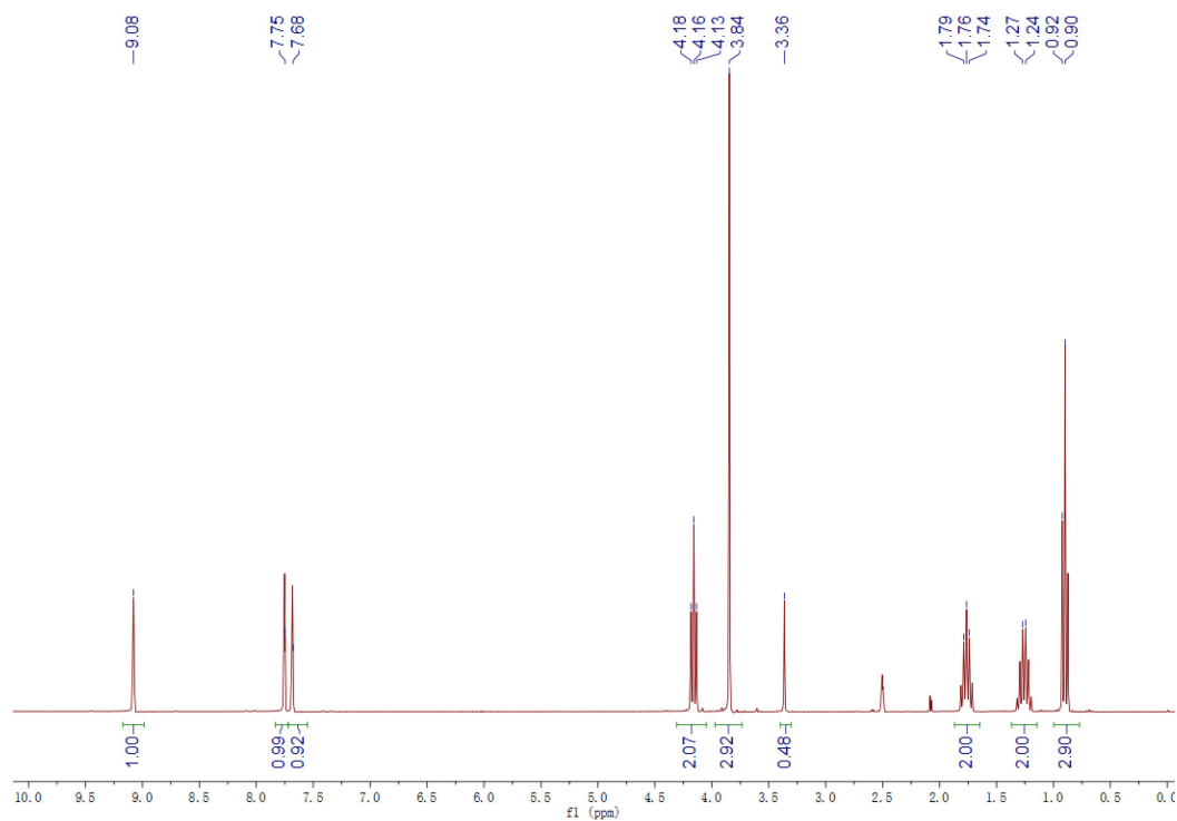
Fig. S3 ^1\text{H} NMR spectrum of [BMIm]DCA
