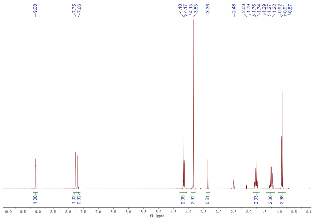
Fig. S5 1 H NMR spectrum of [BMIm]BF 4
