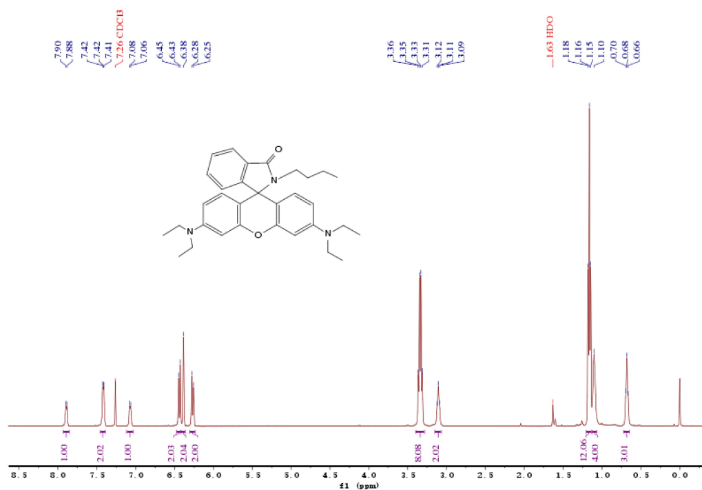
Fig. S7 ^1\text{H} NMR spectrum of intermediate 1
