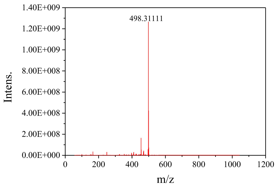
Fig. S8 ESI-MS spectrum of intermediate 1
