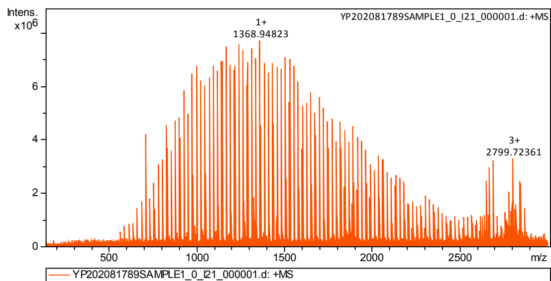
Fig. S1. The results of mass spectrometry experiments of PEI1.8k.
