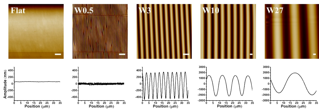
Fig. S1 AFM images taken from side part of substrate and height profiles of the structured PDMS surfaces obtained after imprinting. Scale bar is 4 \mu\text{m} and applies to all images.
