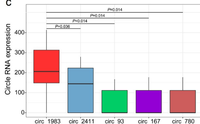
c. Expression of five circRNAs interacting with Gas7 in C_2S -treated BMSCs
