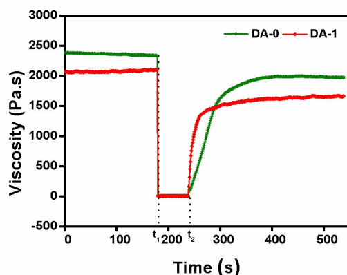
Figure S1 Tactile curve of the slurry of DA-0 and DA-1 group
