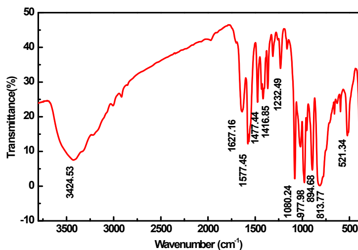
Figure S1. The FT-IR spectrum of compound 1.
