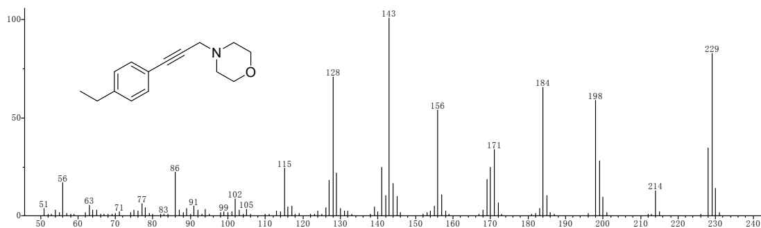
Figure S25. The mass spectrum of product 4j
