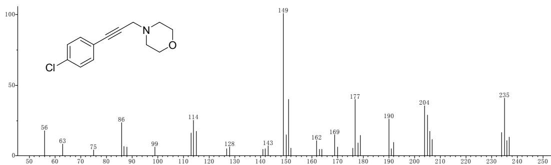
Figure S31. The mass spectrum of product 4m
