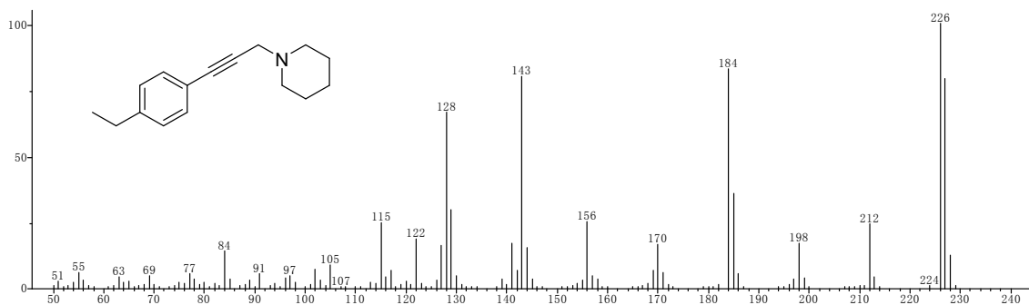
Figure S11. The mass spectrum of product 4c
