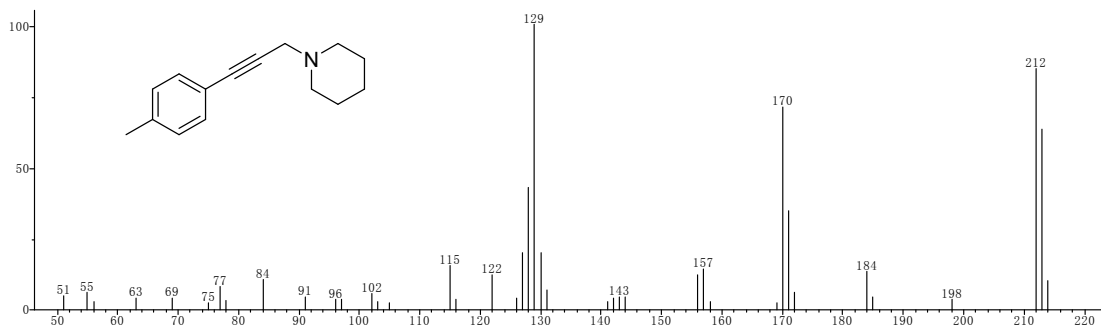
Figure S9. The mass spectrum of product 4b
