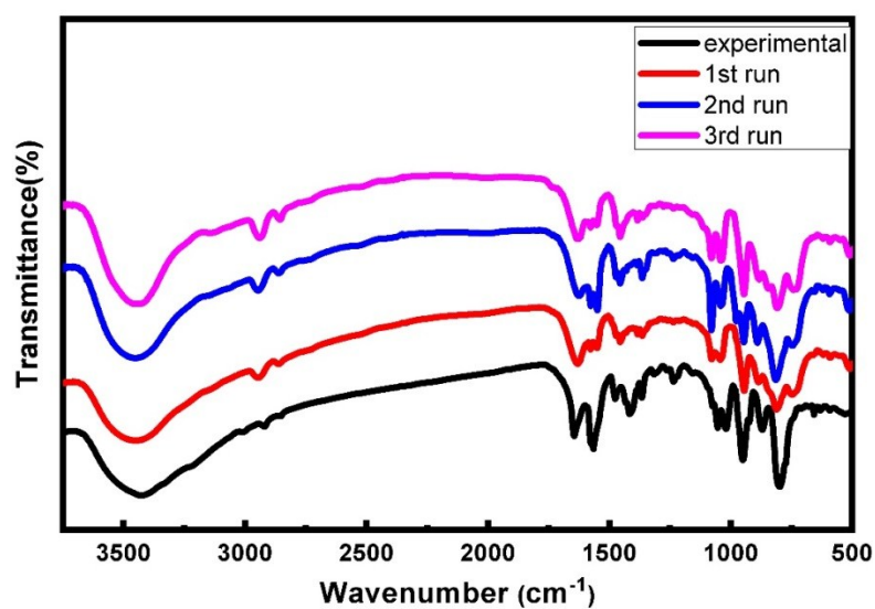
Figure S5. The FT-IR spectra of three runs cycles.
