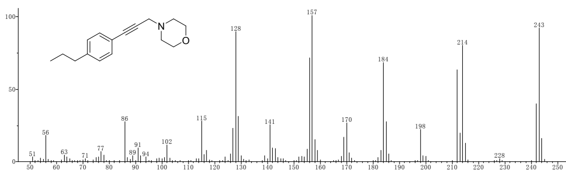
Figure S27. The mass spectrum of product 4k
