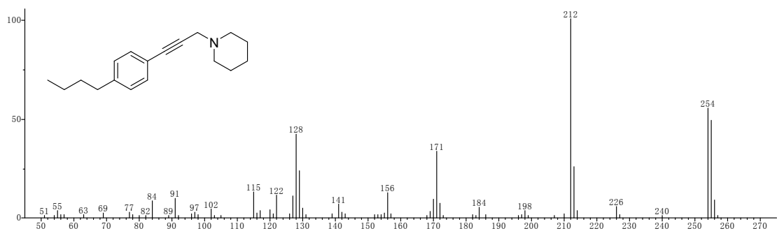
Figure S15. The mass spectrum of product 4e
