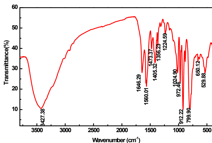
Figure S2. The FT-IR spectrum of compound 2.
