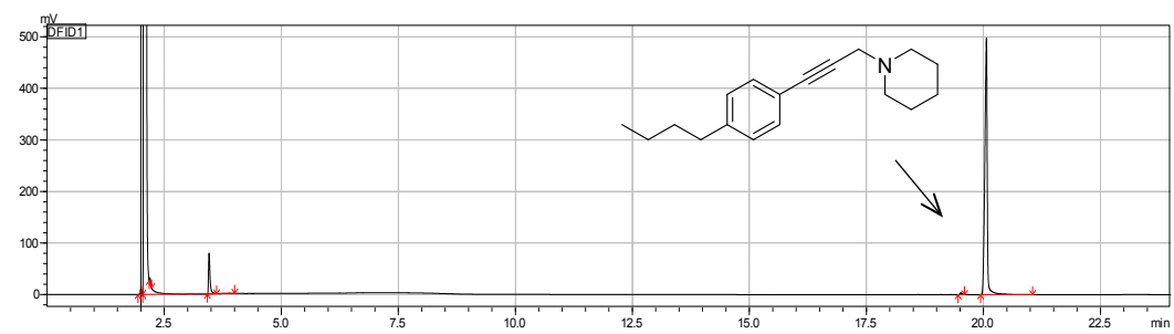
Figure S14. Gas chromatogram of product 4e
