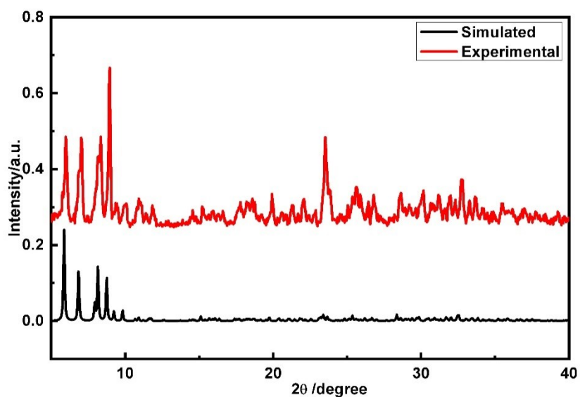
Figure S3. The simulated and experimental PXRD patterns of compound 1.
