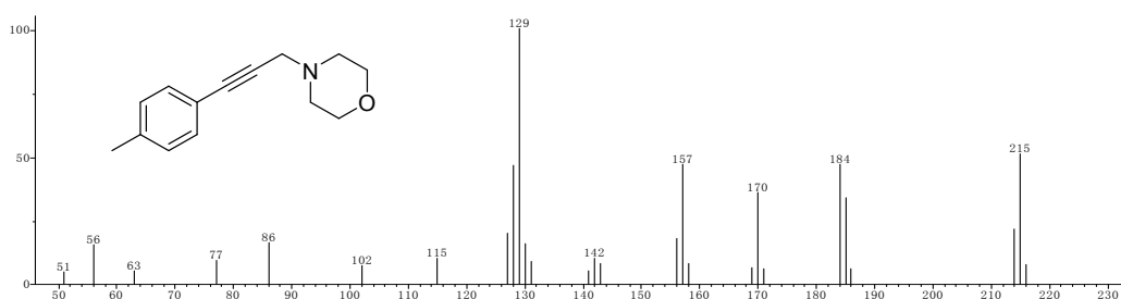
Figure S23. The mass spectrum of product 4i
