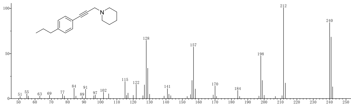
Figure S13. The mass spectrum of product 4d
