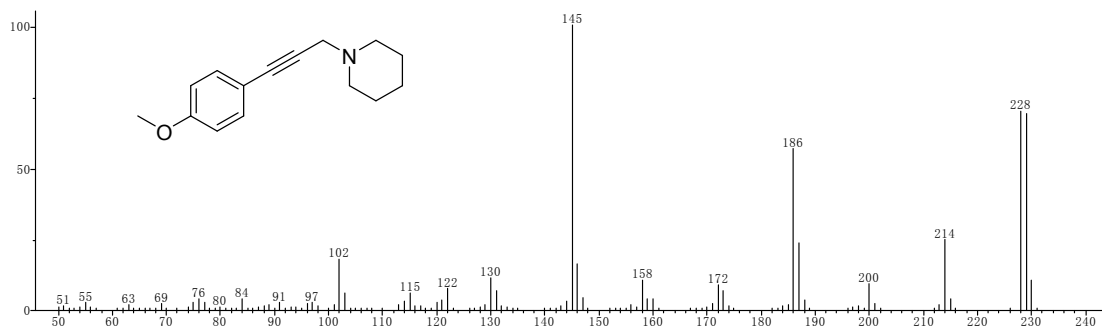
Figure S19. The mass spectrum of product 4g
