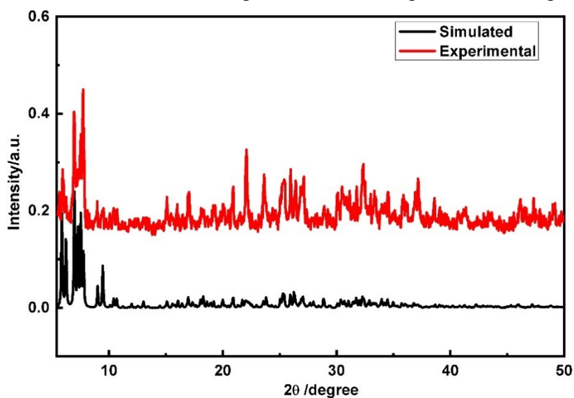
Figure S3. The simulated and experimental PXRD patterns of compound 1.
