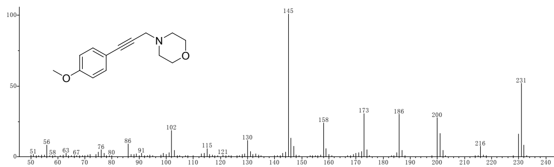
Figure S33. The mass spectrum of product 4n
