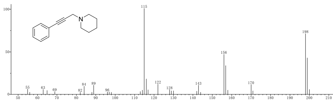
Figure S7. The mass spectrum of product 4a
