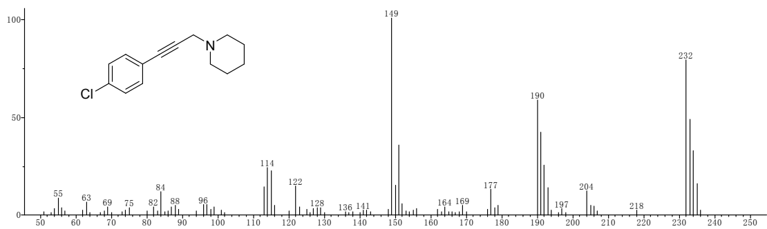
Figure S17. The mass spectrum of product 4f
