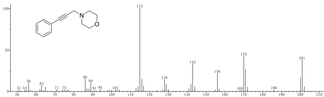
Figure S21. The mass spectrum of product 4h
