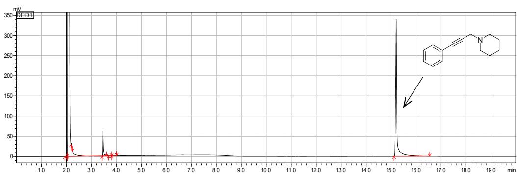
Figure S6. Gas chromatogram of product 4a
