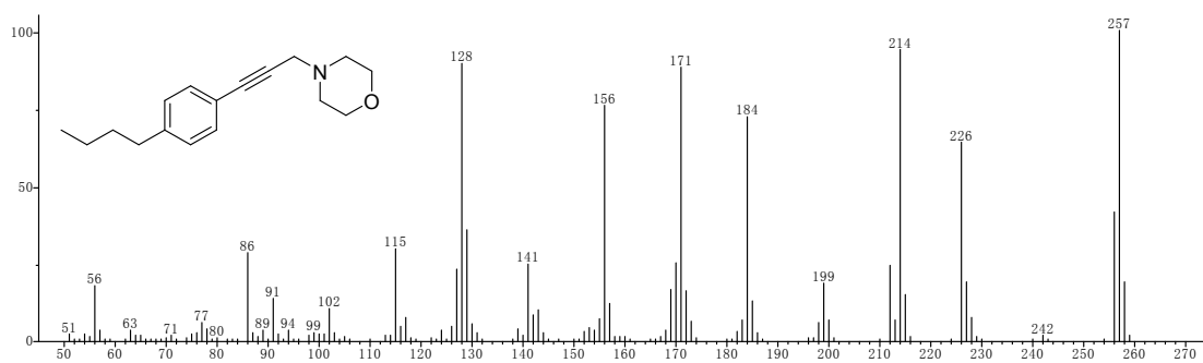
Figure S29. The mass spectrum of product 4l
