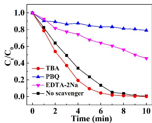
Fig. S3. Active species trapping experiments of BOC-4 for degrade RhB under vis-light irradiation.
