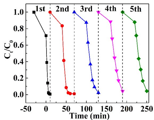
Fig. S4. Durability of BOC-4 for remove RhB.
