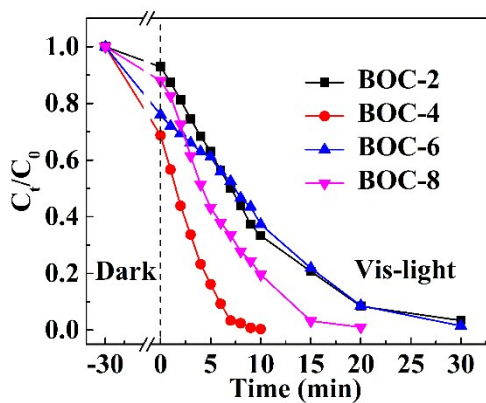
Fig. S2. Photocatalytic activity of the as-prepared samples for the degradation of RhB under vis-light irradiation.
