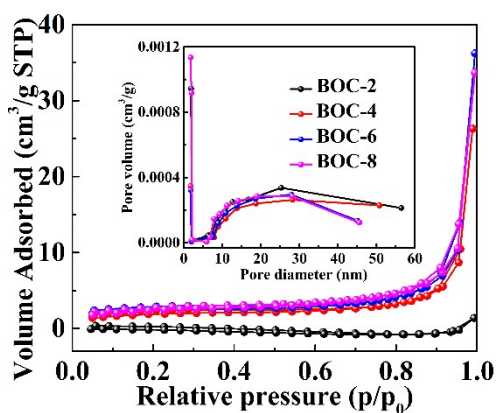
Fig. S1. Nitrogen adsorption-desorption isotherms and the corresponding pore-size distributions (inset) of the as-prepared samples.
