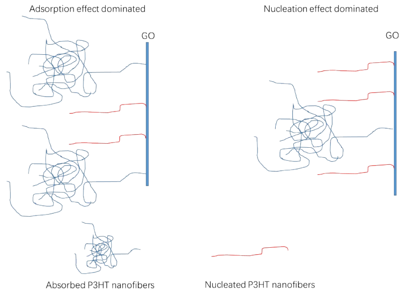
Figure S2. The schematic of the absorbed P3HT nanofibers and nucleated P3HT nanofibers on GO surface.
