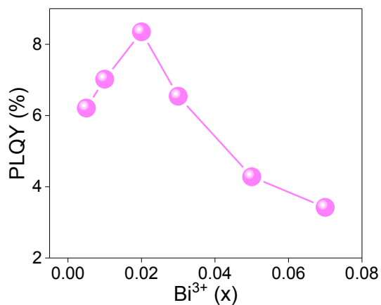
Figure S2. The internal quantum yields of \text{CZBO}:\text{Bi}^{3+} ( x = 0.005, 0.01, 0.02, 0.03, 0.05 ) phosphors.
