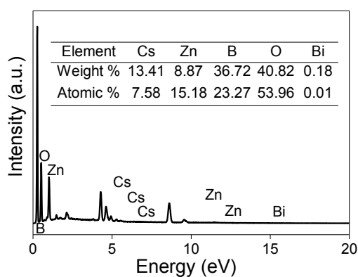
Figure S1 EDX spectrum of \text{CZBO}:\text{0.02Bi}^{3+} sample.
