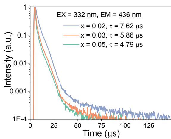
Figure S3. Photoluminescence decay curves of the CZBO:Bi 3+ ( x = 0.02, 0.03, 0.05 ) samples.
