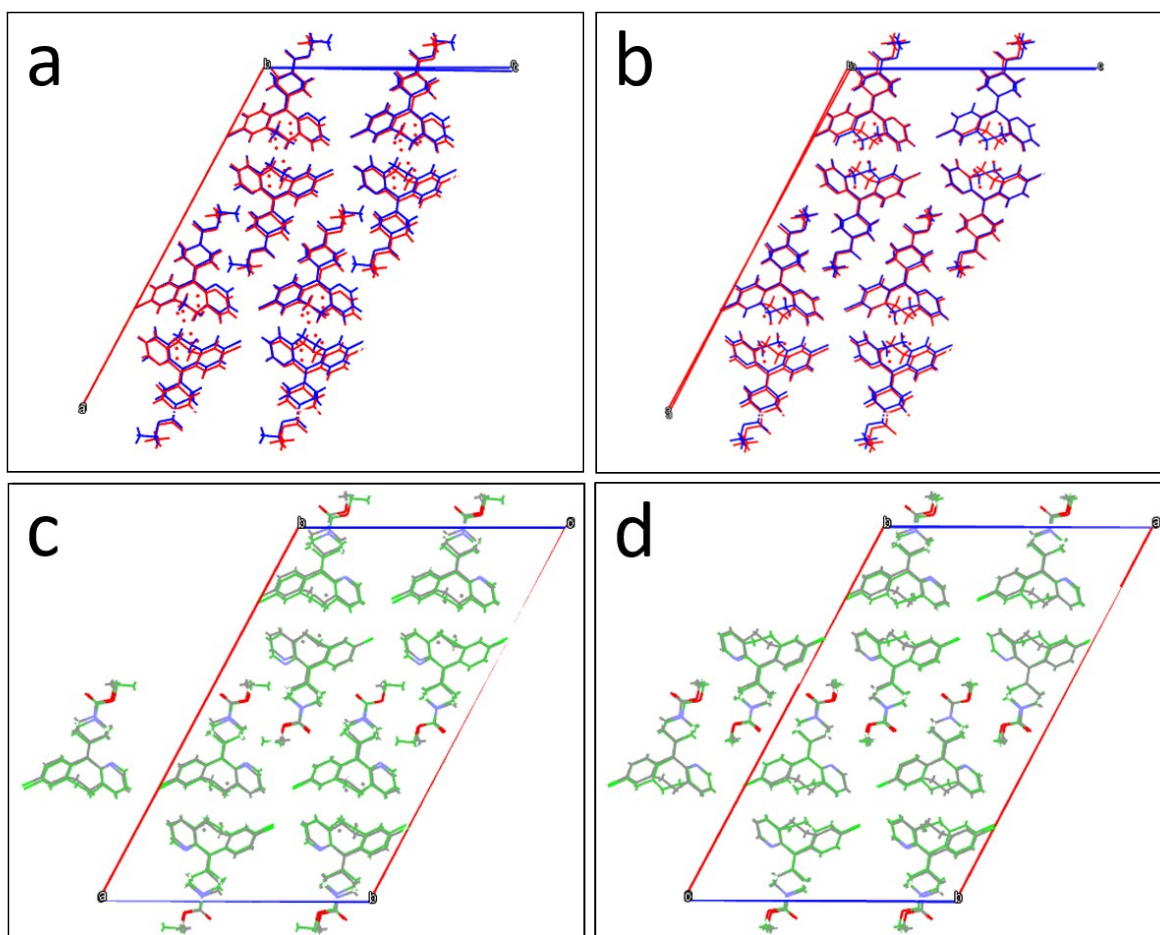
FIGURE S1: ON TOP THE MOLECULAR/STRUCTURAL OVERLAY OF FORM II SA ED STRUCTURE (BLUE) AND SINGLE-CRYSTAL X-RAY STRUCTURE (RED) AND ITS CRYSTAL PACKING SIMILARITY ON THE BOTTOM. TYPE 1 CONFORMATION SHOWN IN (A, C). TYPE 2 CONFORMATION SHOWN IN (B, D).
