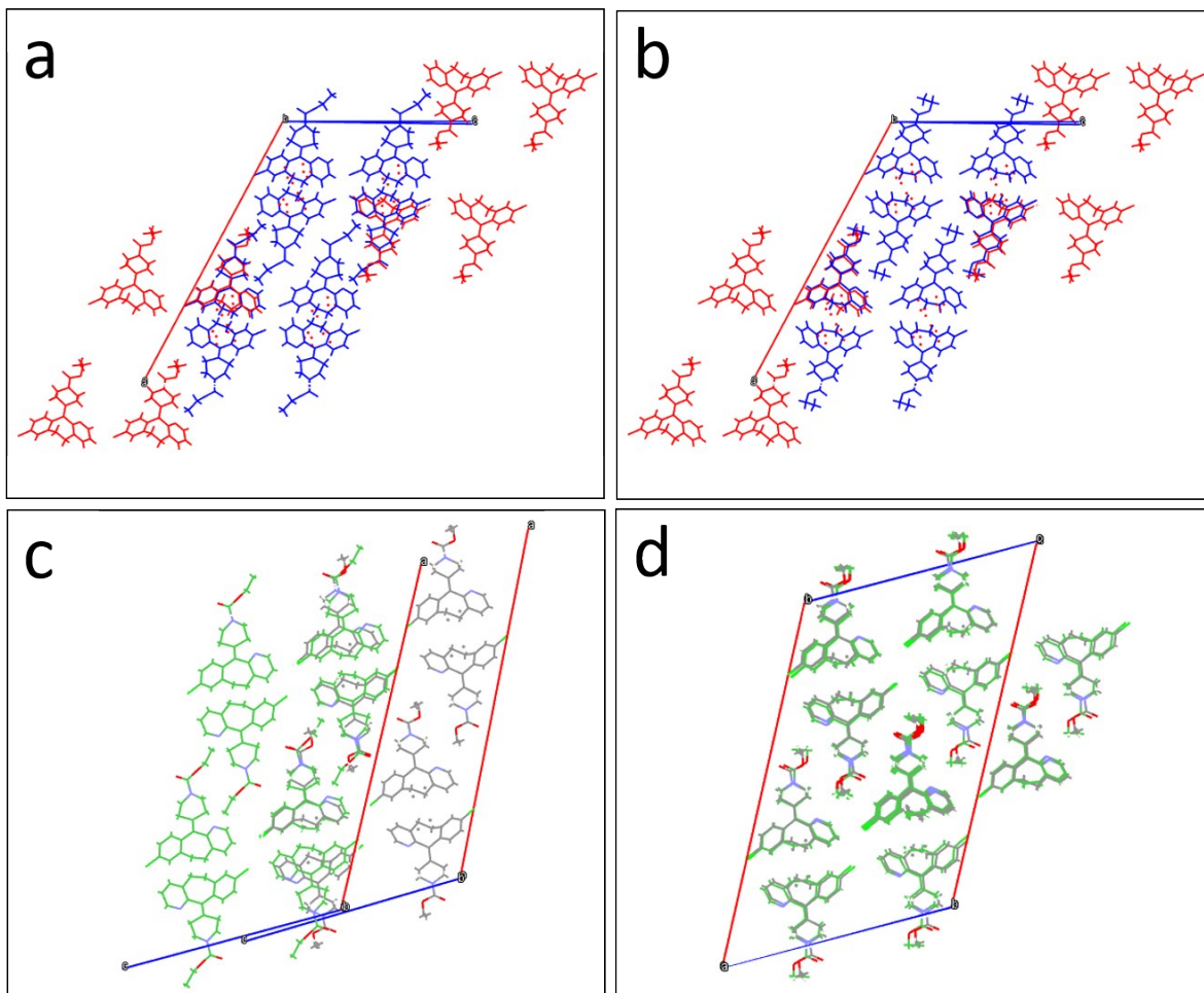
Figure S2: On top molecular/structural overlay of Form II SA ED refined structure (blue) and single-crystal X-ray structure (red) and its crystal packing similarity on the bottom. Type 1 conformation shown in (a, c). Type 2 conformation shown in (b, d).
