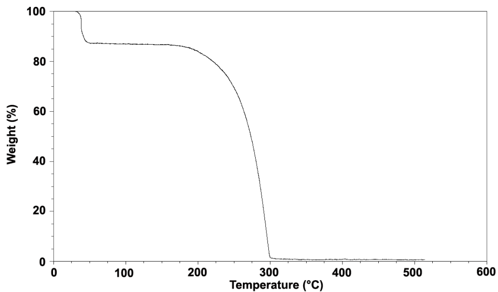
Figure S1 Thermogram of L1.
