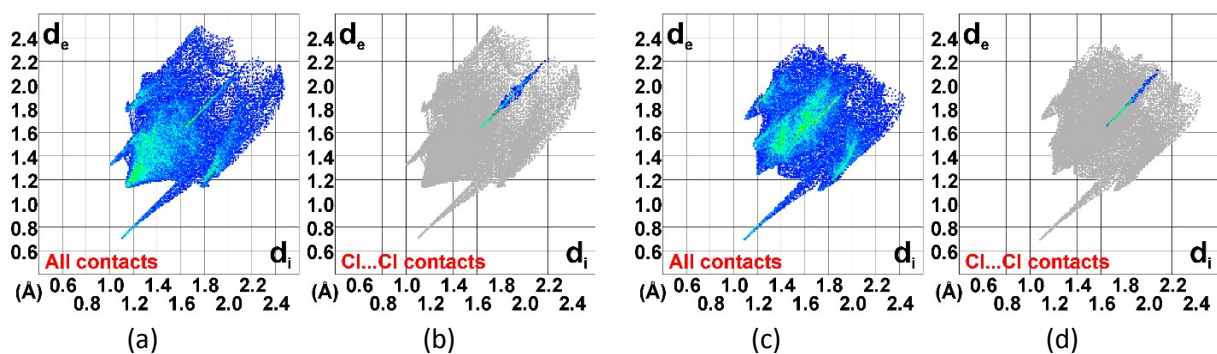
Hirshfeld fingerprint plots for a) 4-chloropiperidine monohydrate at 100 K , all contacts b) 4-chloropiperidine monohydrate at 100 K , the Cl...Cl contacts, c) 4-chloropiperidine trihydrate at 100 K, all contacts b) 4-chloropiperidine trihydrate at 100 K , Cl...Cl contacts.
