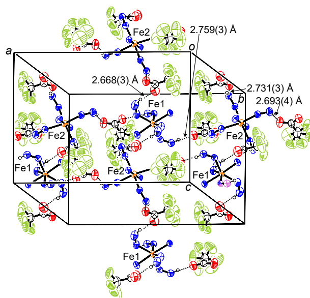
Fig. S1 3D hydrogen bond network of 1 at 300 K.
