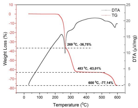
Fig. S3 TG-DTA profiles of 1.
