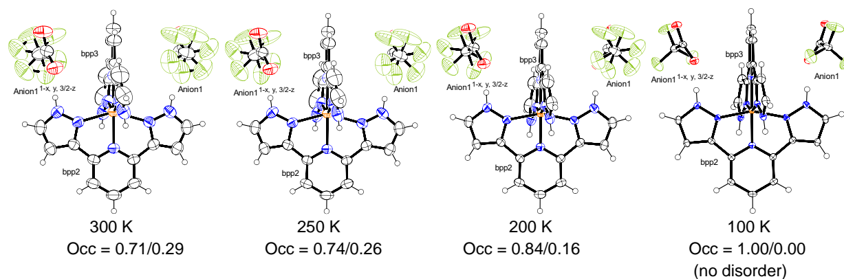
Fig. S2 A projection normal to the bpp2 plane.
