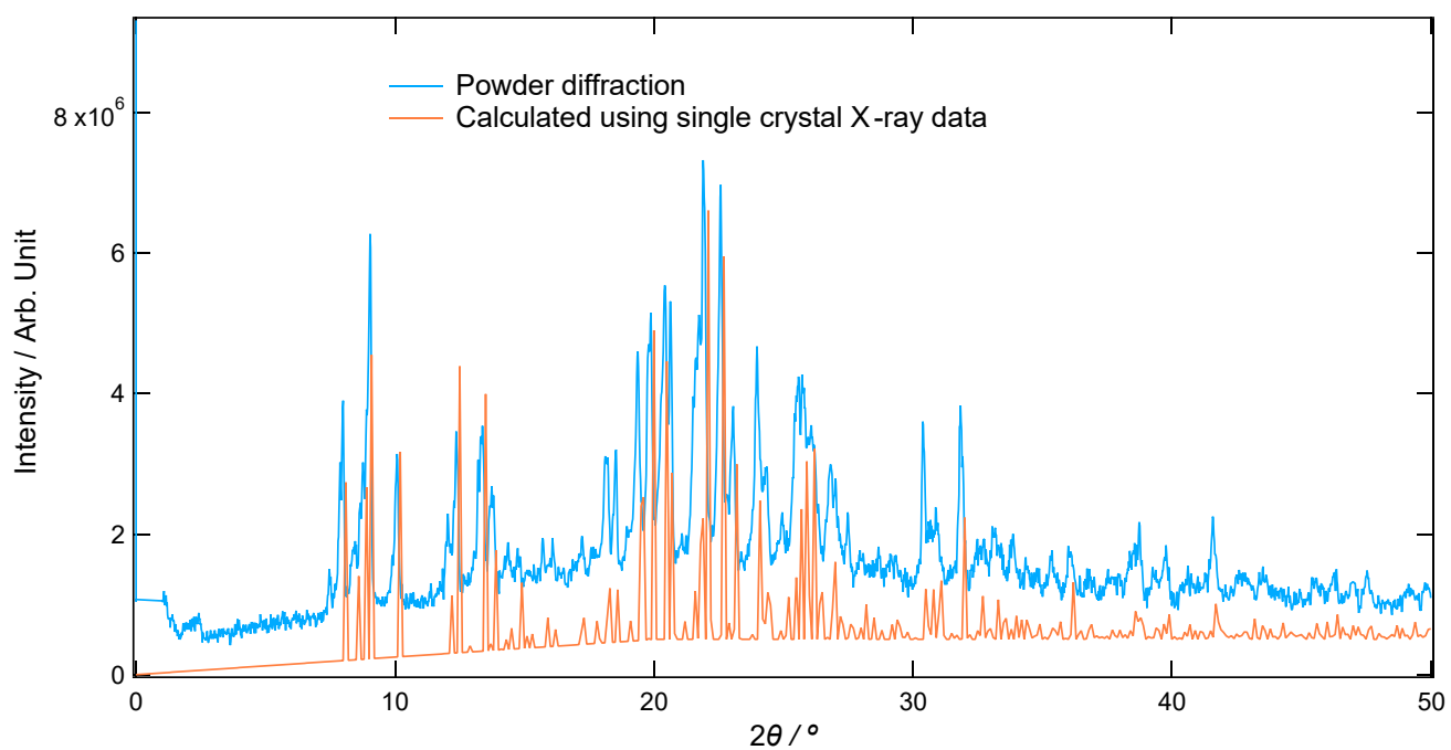
Fig. S4 Powder X-ray diffraction of 1 with the estimated powder diffraction using single crystal X-ray data.
