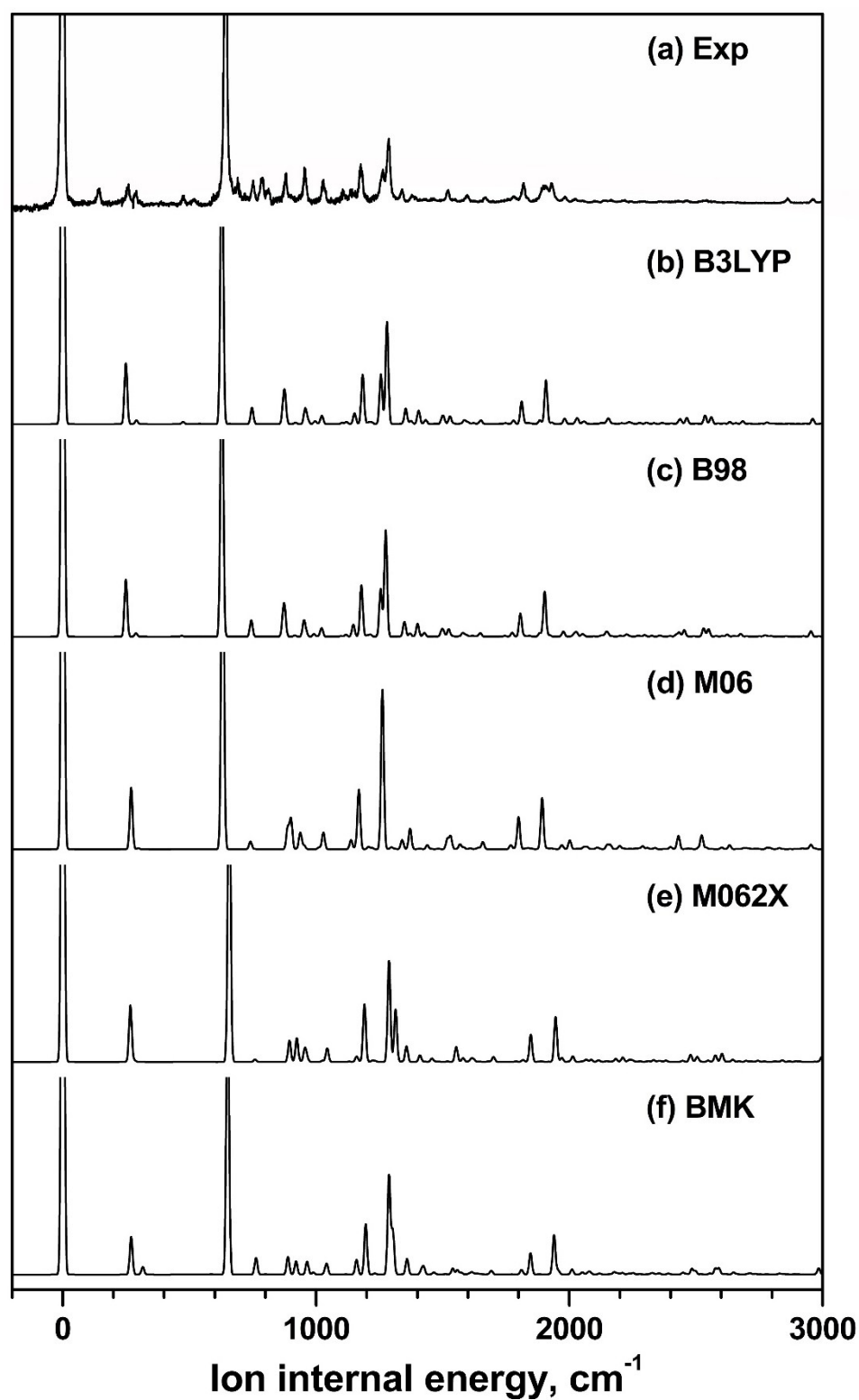
Figure S1 (a) VUV-MATI spectrum of THT. Simulated spectra using the Franck-Condon factors and the vibrational frequencies calculated at the (b) B3LYP, (c) B98, (d) M06, (e) M062X, and (f) BMK levels with cc-pVTZ basis set for the C 2 conformer. All spectra are magnified by fourfold for detailed comparison.
