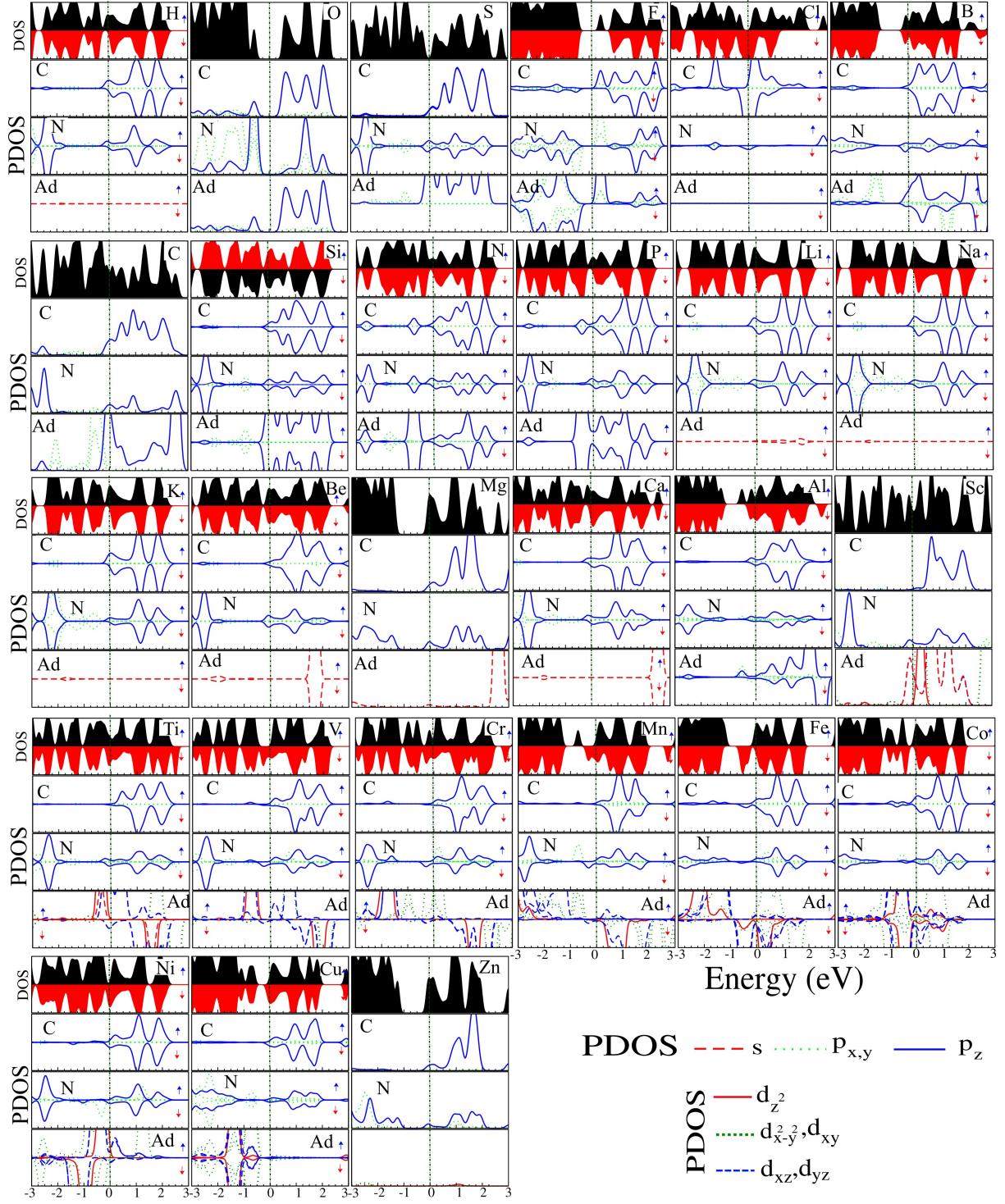
Figure 1: DOS and PDOS of different atoms embedded into the holey site of the C_6N_8 monolayer. The zero of energy is set at E_F .
