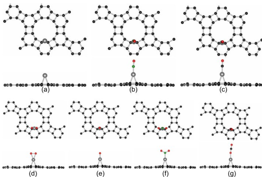
Fig. S1 The stable geometries for (a) Cu-graphenylene and (b) NO, (c) CO, (d) O 2 , (e) O, (f) NO 2 , (g) CO 2 adsorbed at Cu-graphenylene sheet, respectively. Black, gray, green and red balls represent the C, Cu, N and O atom, respectively.
