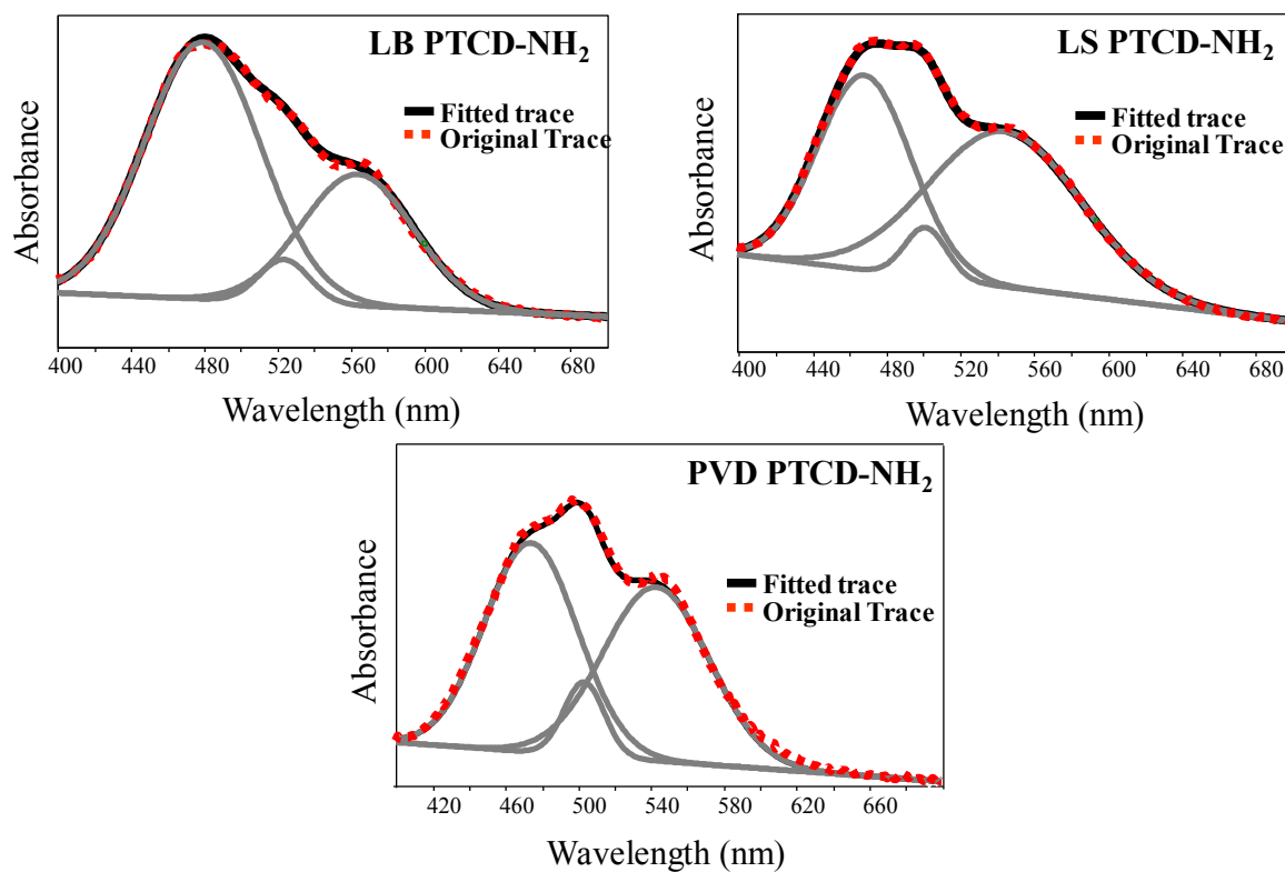
Fig. SI-1 UV-Vis absorption spectra for PTCD-NH 2 LB, LS, and PVD films: original trace, fitted trace, and peaks using Gaussian function (software GRAMS AI).
