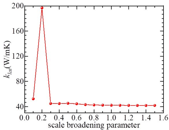
Fig. S2: The convergence tests of \kappa_{lat} for different scale broadening parameters with 200x200x1 q-grid at 300 K.
