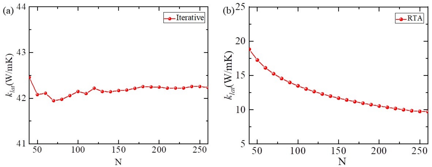
Fig. S1: (a) The convergence tests of \kappa_{lat} for the iterative solution with different q-grid at 300 K. (b) The convergence tests of \kappa_{lat} for RTA solution with different q-grid at 300 K.
