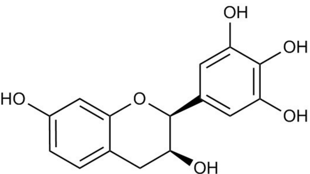
Epigallocatechin
