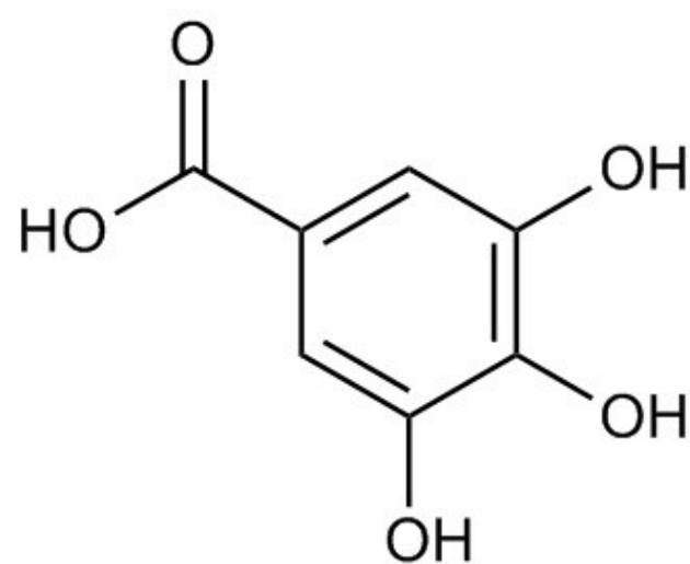
Gallic Acid
